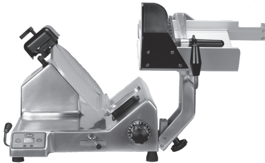
Figure 12-3 Cleaning Position
