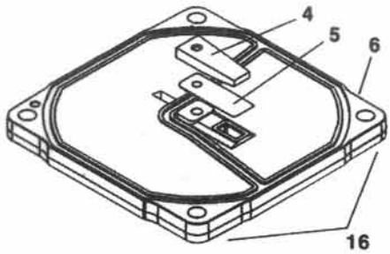
Valve Plate Assembly (available separately) (Valve Plate Assembly also includes items 7 & 8, as shown in the main exploded view)
